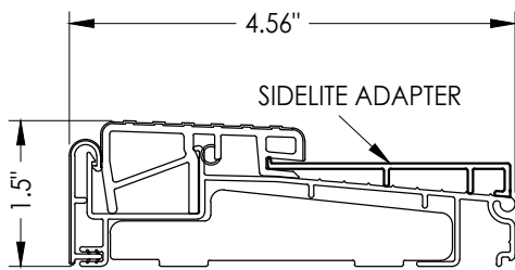
T15 OUTSWING THRESHOLD w/ SIDELITE ADAPTER
